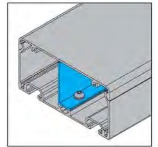
Partition profile-16x48
