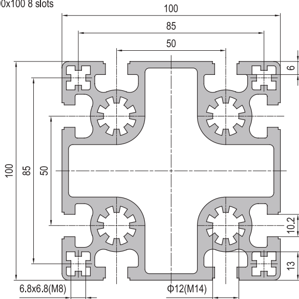
100x100 8 slots
