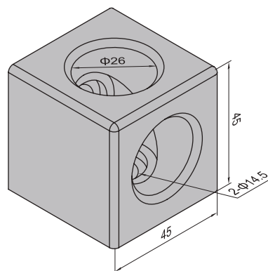
Cubic Connector-4545-2
