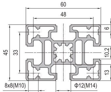
45x60 4 slots
