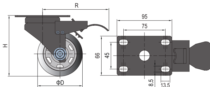
Castor-Plate-Brake
