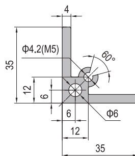
Angle Profile 35x35x4
