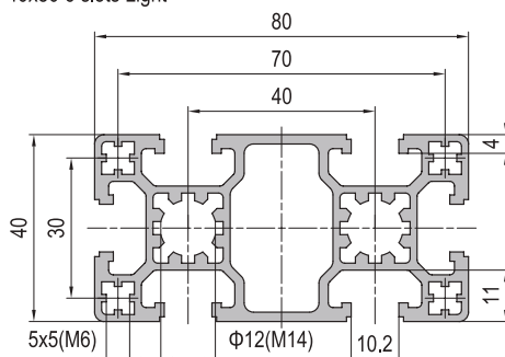
40x80 6 slots Light
