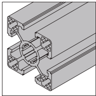
40x40 4 slots Super Light
