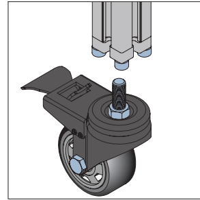
Castor-Plate-Universal-Heavy
