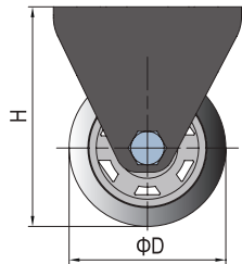
Castor-Plate-Brake
