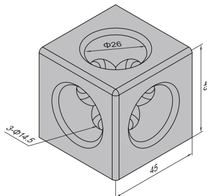
Cubic Connector-4545-3
