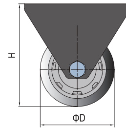
Castor-Plate-Fixed-Heavy
