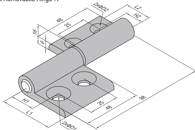
Al Removable Hinge-R
