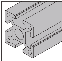
40x40 4 slots Heavy
