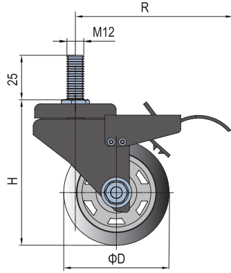
Castor-Thread-Brake
