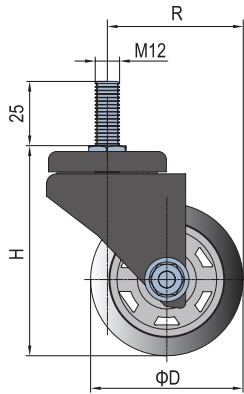
Castor-Thread-Universal
