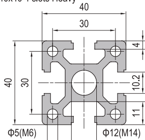
40x40 4 slots Heavy
