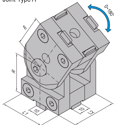
Joint-Type B
