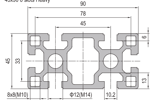
45x90 6 slots Heavy
