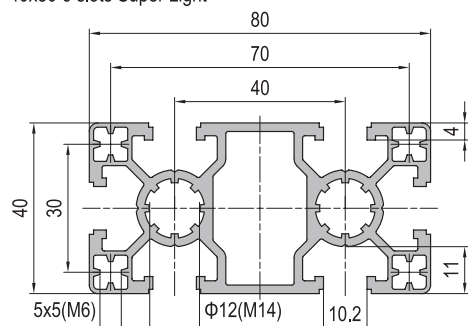
40x80 6 slots Super Light
