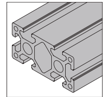
40x80 6 slots Heavy
