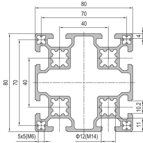
80x80 8 slots
