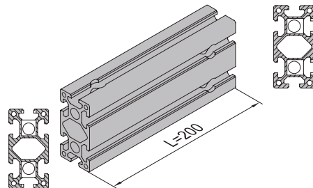
Example B: 1. 11. 40.040080.08H-200-LDV/RDH
