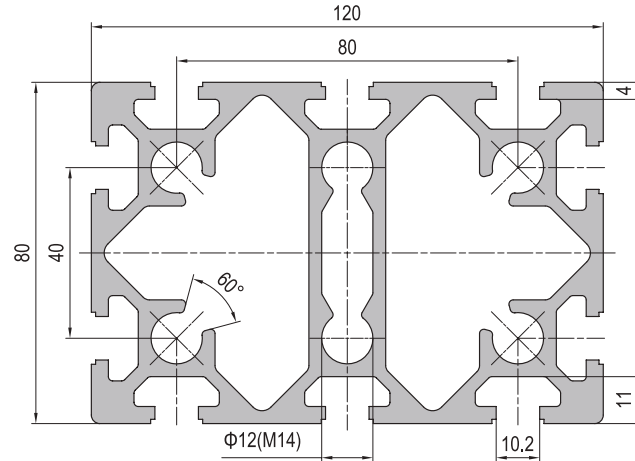
80x120 10 slots
