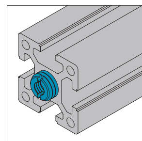
Hole Reducer Bolt M14/M8 PG40/PG45/PG50/PG60 with core hole-Φ12(M14)
