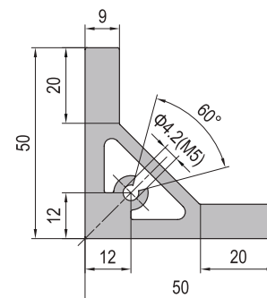
Angle Profile 50x50x9
