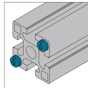
Hole Reducer Bolt M10/M6 PG45 with square corner hole-8x8(M10)
