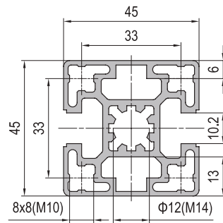
45x45 2 slots Type B
