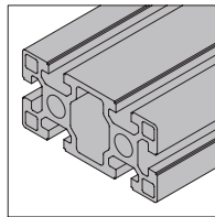
45x90 6 slots Heavy
