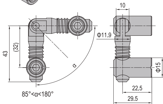
PG45-Miter (Model C)
